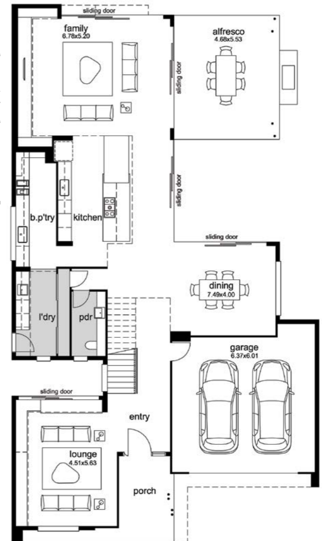
LOWER FLOOR PLAN 250.66sq.m.
