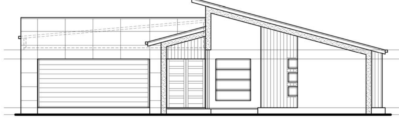
front elevation ————— waterline elevation
