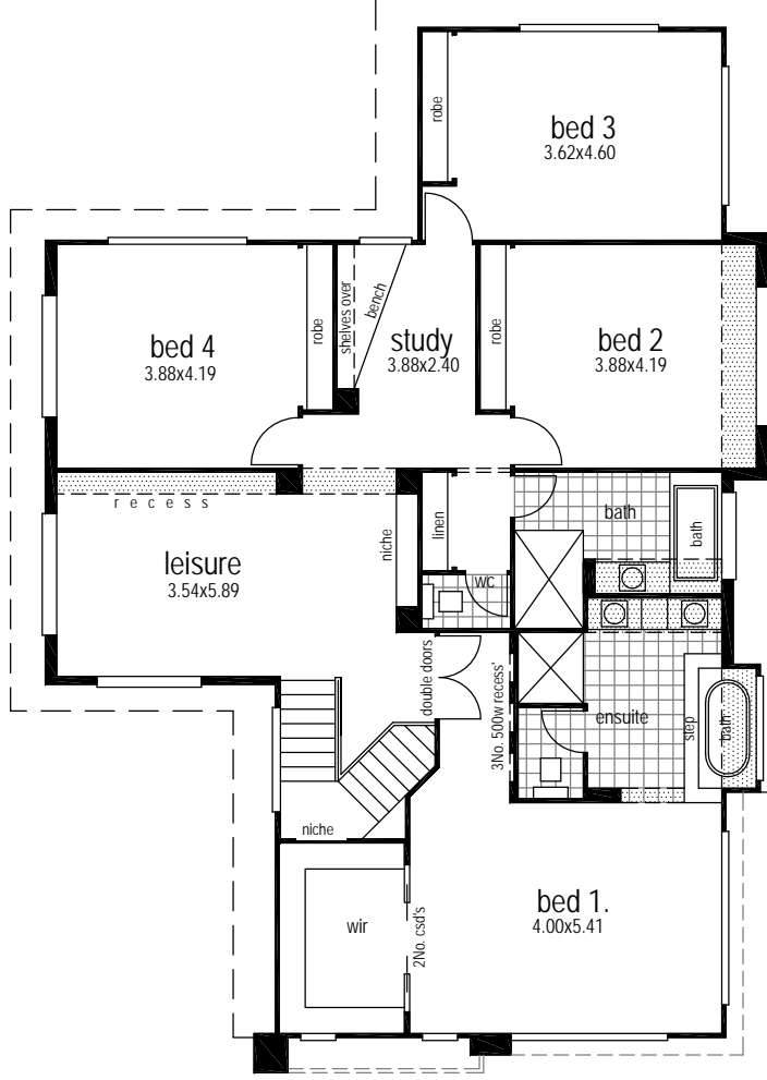
upper floor plan 168.25sq.m.
